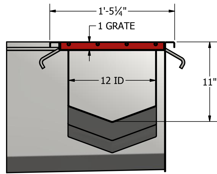
SECTION B-B SHALLOW POINT
