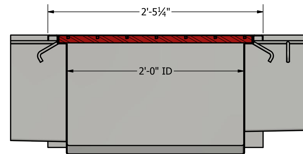
SECTION E-E
