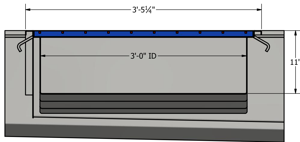
SECTION C-C SHALLOW END
