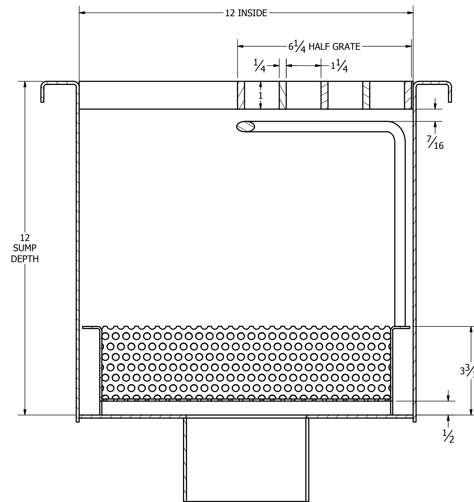
SECTION A-A SCALE 1 / 2
